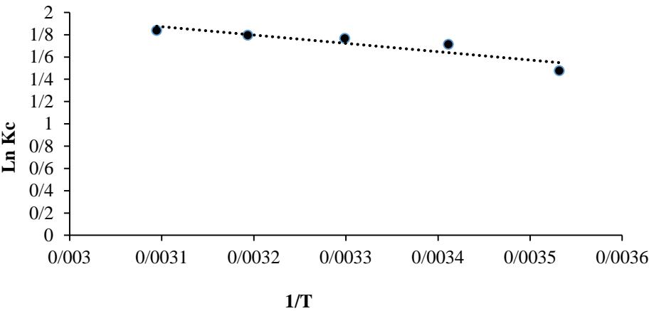
Figure 10. Thermodynamic diagram of diclofenac adsorption
